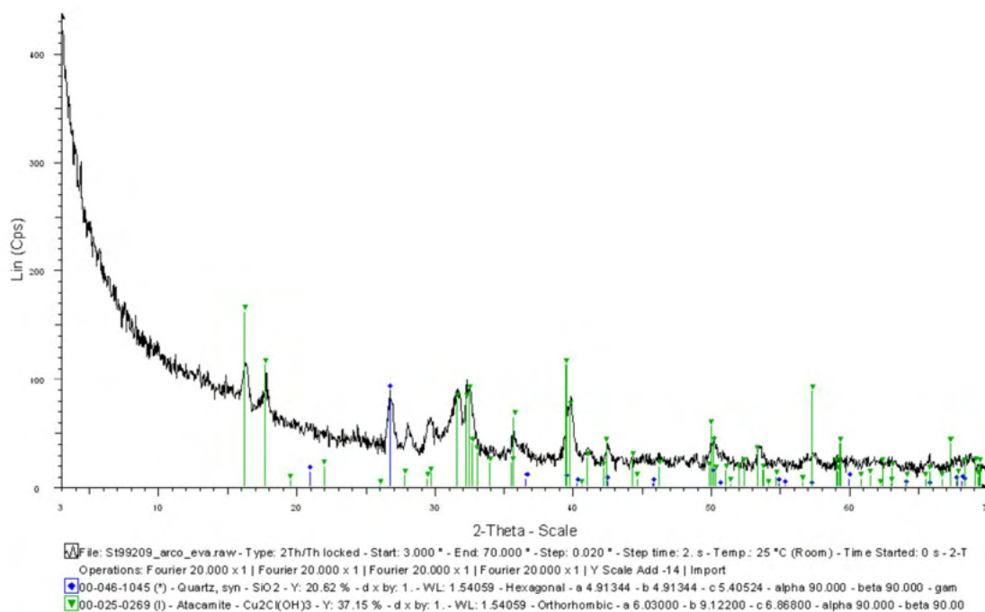
Figure 184. Diffractogram of a point of the bow of the fibula inv. no. St. 99209 (Forcello di Bagnolo San Vito): atacamite (green) and quartz (blue).
