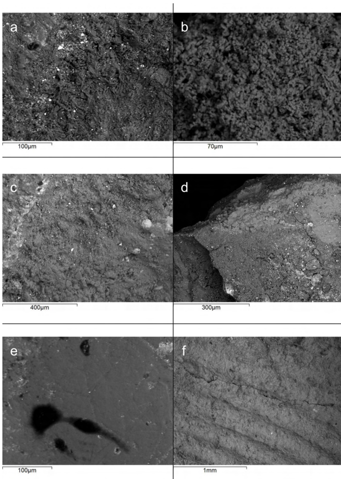
Figure 154. a) BSE-image of a circular decoration (Motto Lagone, T1): multi-branched micro-morphology; b) BSE-image of a circular decoration (Bra Museum, inv. no. M589/3): micro-porous morphology; c) BSE-image of a circular decoration (Novara Museum, inv. no. 946): mammellonary micro-morphology; d) BSE-image of a sample from a circular decoration (Brignano Frascata, inv. no. C-FR-S/2): crusty micro-morphology; e) BSE-image of a circular decoration (Motto Lagone, T1): compact micro-morphology; f) BSE-image of an element of a composite bow fibula (Brembate Sotto, inv. no. 3052): crenulation features.
