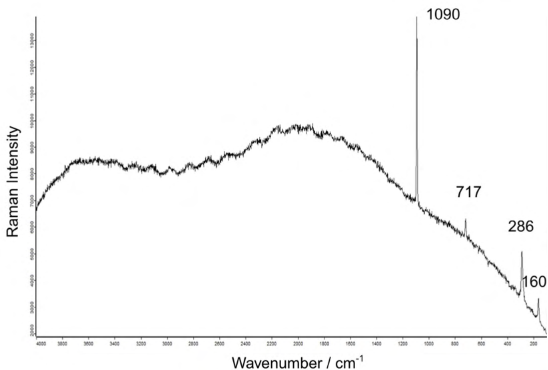
Figure 102. Raman spectrum of fossil coral from Piedmont (r_fc_P): calcite; green laser 532 nm, extended range, 6 seconds for 6 cycles, 10x magnification, D0.6 filter.
