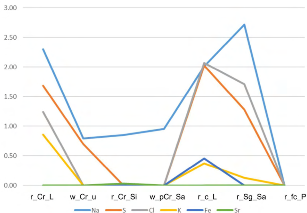
Figure 112. Graph of the occurrence of some minor elements (Na, S, Cl, K, Fe, Sr) in different samples [r_Cr_L: unworked ligurian C. rubrum ; w_Cr_u: worked-polished C. rubrum ; r_Cr_Si: sicilian C. rubrum collected on the beach; w_pCr_Sa: sardinian pinkish-to-white worked coral; r_c_L: Ligurian white coral; r_Sg_Sa: Sardinian S. gaederopus ; r_fc_P: Piedmont fossil coral].
