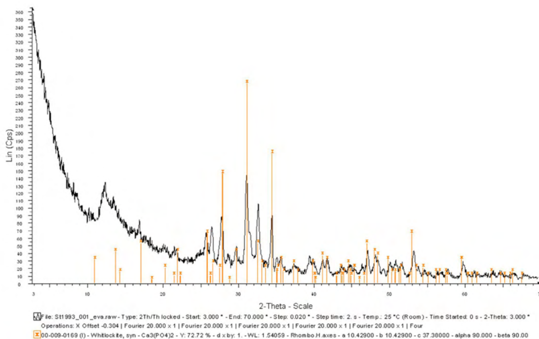
Figure 147. Whitlockite diffractogram of the sample inv. no. St. 1993 (Como, Ca' Morta).
