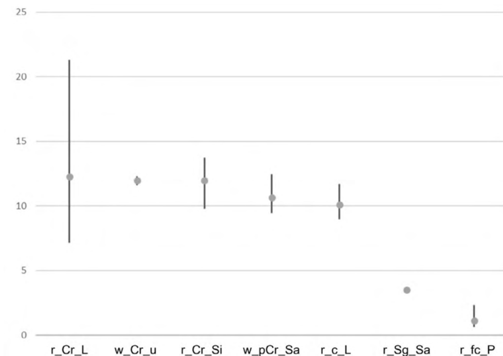
Figure 111. Mg-content variation in each sample (bar indicates the variation between minimum and maximum value) and average value (point indicates the average value of all the points of analysis on the sample) [r_Cr_L: unworked ligurian C. rubrum ; w_Cr_u: worked-polished C. rubrum ; r_Cr_Si: sicilian C. rubrum collected on the beach; w_pCr_Sa: sardinian pinkish-to-white worked coral; r_c_L: Ligurian white coral; r_Sg_Sa: Sardinian S. gaederopus ; r_fc_P: Piedmont fossil coral].
