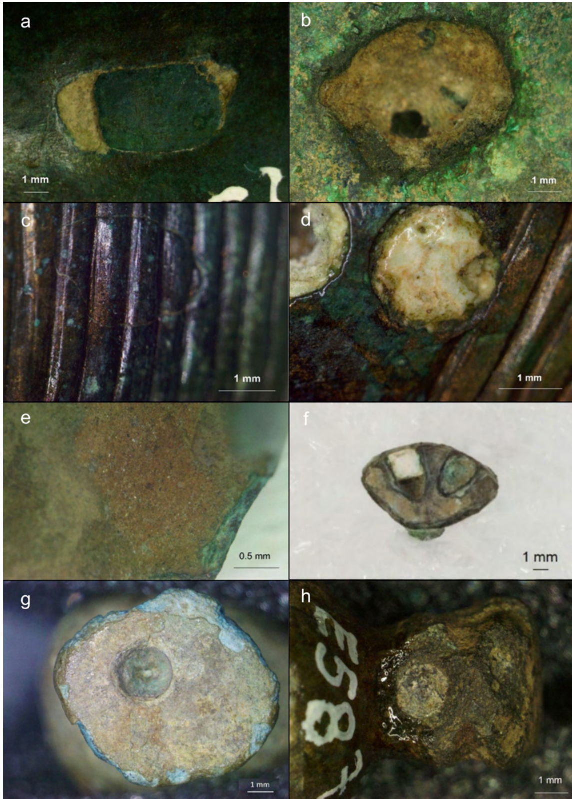
Figure 200. a) Detail of the ventral-face gusset (inv. no. St. 57216, Como); b) Detail of the ventral-face residual hole of the gusset (inv. no. E5552, Como); c) Detail of the upper face of the bow and the point of emergence of the spring-side 'support': linear decoration in continuity (tomba 1, Motto Lagone, Arona); d) Detail of the upper face of the arch: the circular decoration covers the linear one, with a wax coating (tomba 1, Motto Lagone, Arona); e) Detail of the core mixture (inv. no. St. 57220, Como); f) Section of a full-arch fibula: detail of the inset in the hole (inv. no. Sp834, Villa del Foro); g) Foot termination drilled after casting (inv. no. 23-M380-9.4, Castello di Annone); h) Coarse foot termination (probable casting funnel; inv. no. E5873, Como).
