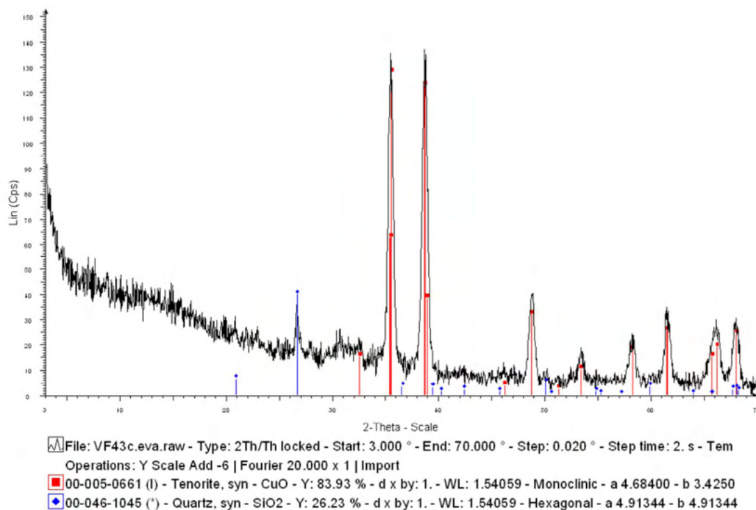
Figure 183. Diffractogram of sample VF43c, collected on fibula inv. no. SP28b (Villa del Foro): tenorite (red) and quartz (blue).
