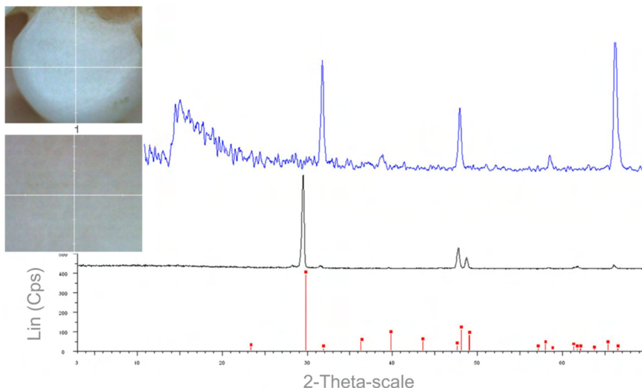
Figure 140. Comparison of diffractograms obtained from the same piece of modern C. rubrum (w_pCr_Sa). The object is perfectly flat on one side and worked on the other. The diffractogram obtained from the flat side (in black) is of considerably better quality and shows the presence of the Mg-calcite peaks (in red). The one collected on the worked side (in blue) shows the irregular background and a consequent shift of the calcite peaks.
