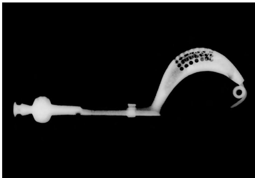
Figure 201. Leech fibula with terracotta core from Tomb 1 of Motto Lagone (Arona).
