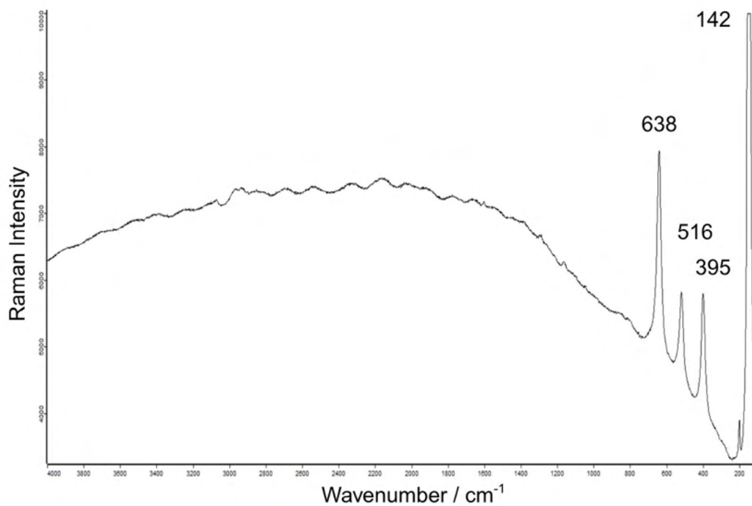
Figure 128. Raman spectrum of whitish decoration on a fibula from Parre (inv. no. 40; magnification 10X, filter d 0.3): anatase.
