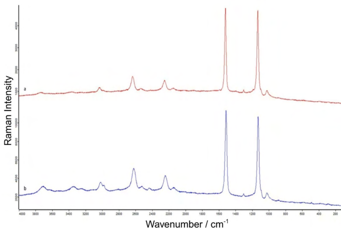
Figure 93. Raman spectra of C. rubrum in red and S. gaederopus in blue, acquired with green laser (532 nm).
