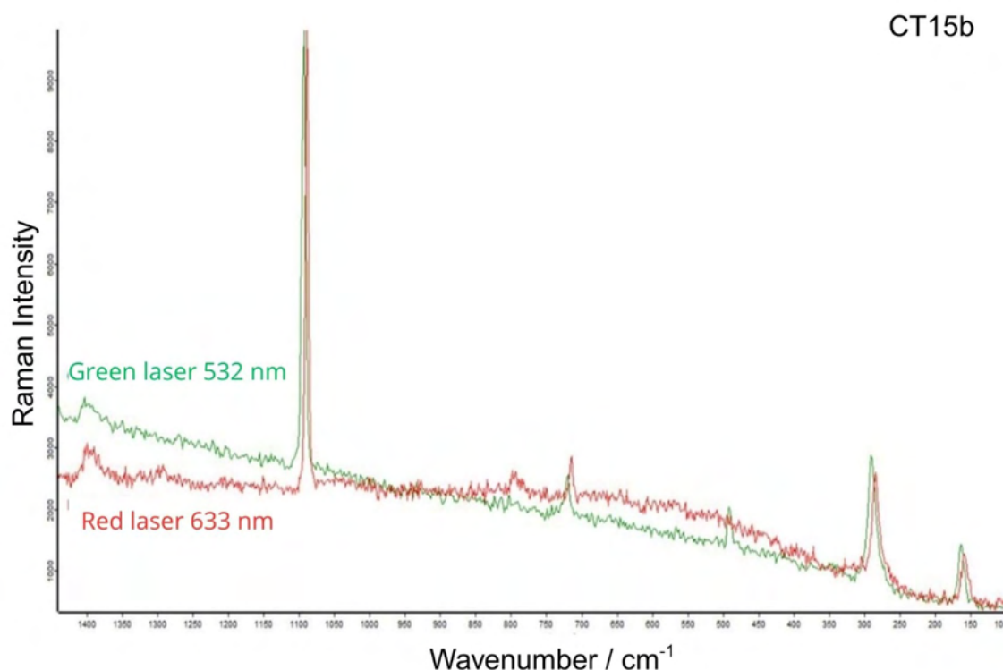
Figure 92. Raman spectra of the same sample (CT15b) with green laser (532 nm) in green and with red laser (633 nm) in red: small peak shift is evident using different lasers.
