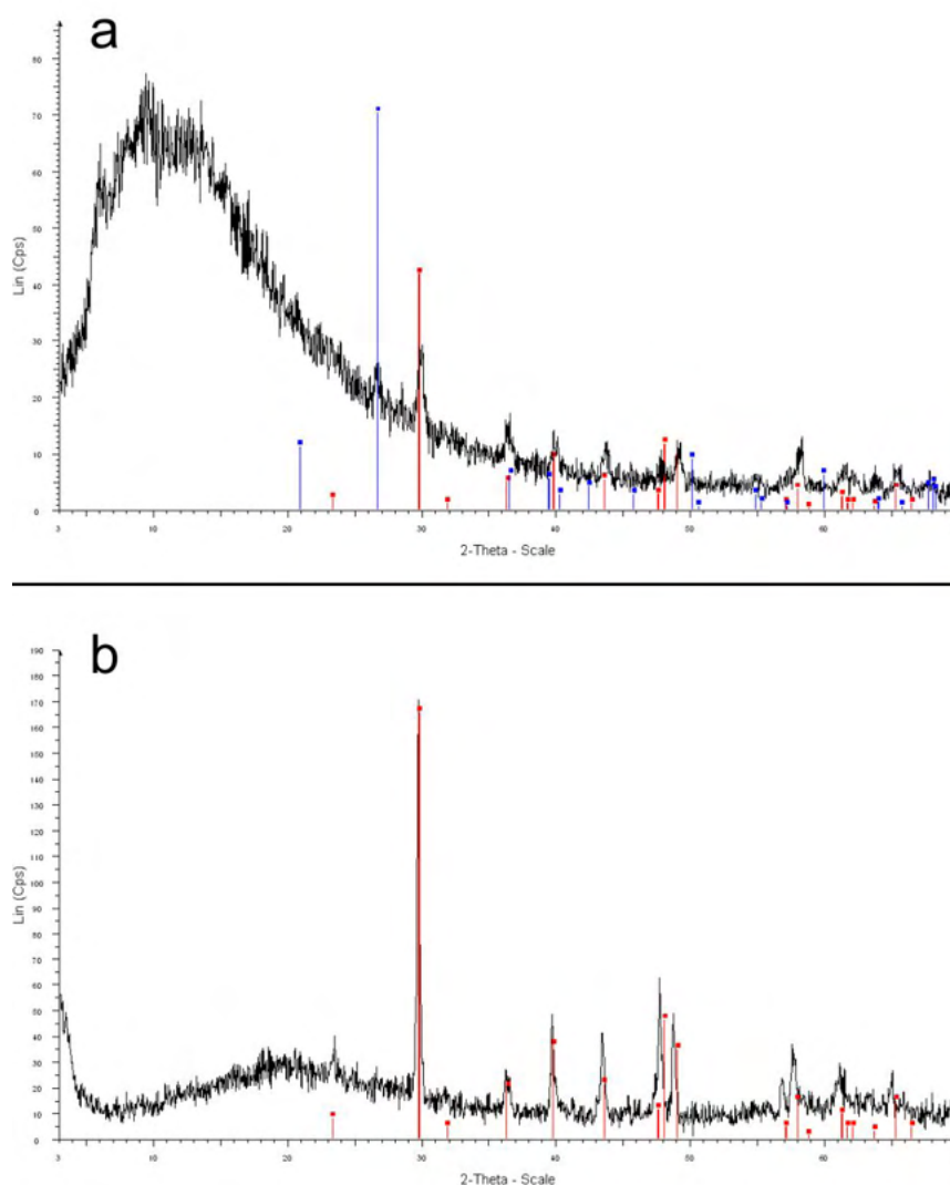
Figure 139. Comparison of diffractograms of samples collected from finds (a) inv. no. C-FR-NE/2 (Brignano Francata, leech fibula with circular decoration) and (b) 22.S288-1.205 (Golasecca, loc. Galliasco, leech fibula with circular decoration), analysed by micro-area XRD (left) and XR Powder Diffraction (right), respectively.
