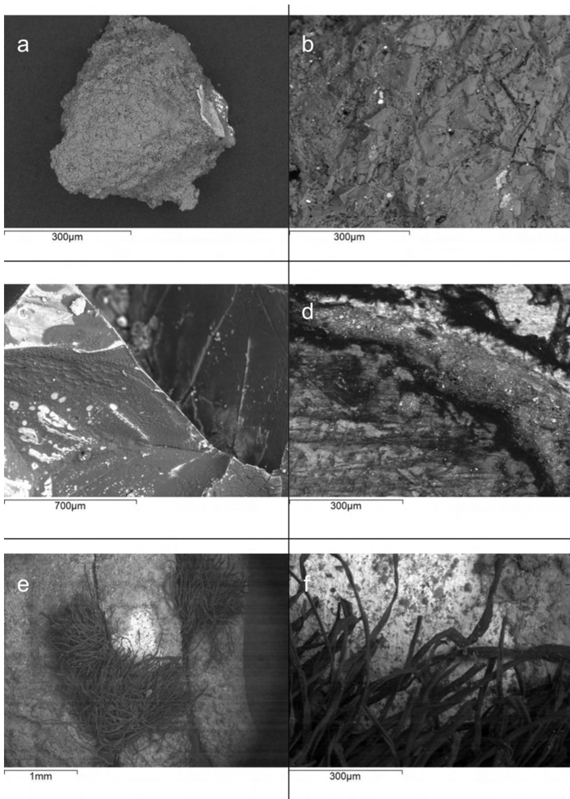
Figure 222. a) BSE-image of a sample from a circular decoration (Brignano Frascata, inv. no. C-FR-NE/2): mammellony micro-morphology; b) BSE-image of a vitreous bead (Motto Lagone, grave 1): conchoid micro-morphology; c) BSE-image of a vitreous bead (Castelletto Ticino, inv. no. CT14031X, CT868c): high presence of Paraloid on the surface; d) BSE-image of a circular decoration (Como, via Isonzo, inv. no. St.57220): detail of the presence of incoherent material standing between the inset and the border of the hole containing it; e) BSE-images of Longone al Segrino type pendant (Castelletto Ticino, inv. no. D1750): detail of the presence of fibre residues trapped in the bronze rod spring; f) BSE-images of Longone al Segrino type pendant (Castelletto Ticino, inv. no. D1750): detail of the presence of fibre residues trapped in the bronze rod spring.
