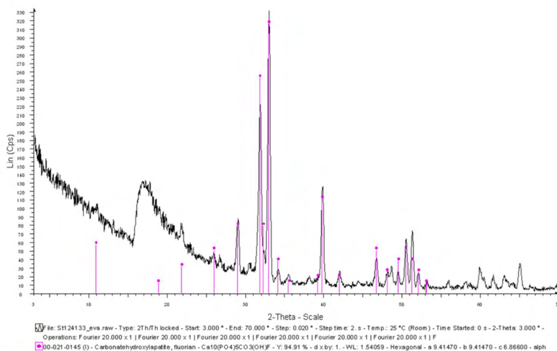
Figure 146. Carbonate-hydroxylapatite diffractogram of the sample St. 124133 (Como, Ca' Morta) with background rise, but no peak shift.
