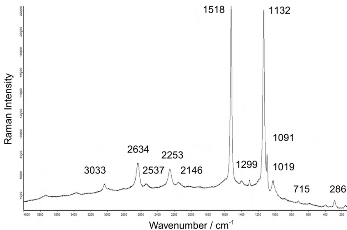
Figure 118. Raman spectrum of whitish circular decoration on Motto Lagone leech-fibula (magnification 20X, filter d 0.3): polyenes and calcite.
