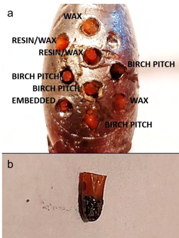
Figure 205. a) test 6: evidence of coral embedding with different binders; b) failed embedding of coral inset held by birch pitch.
