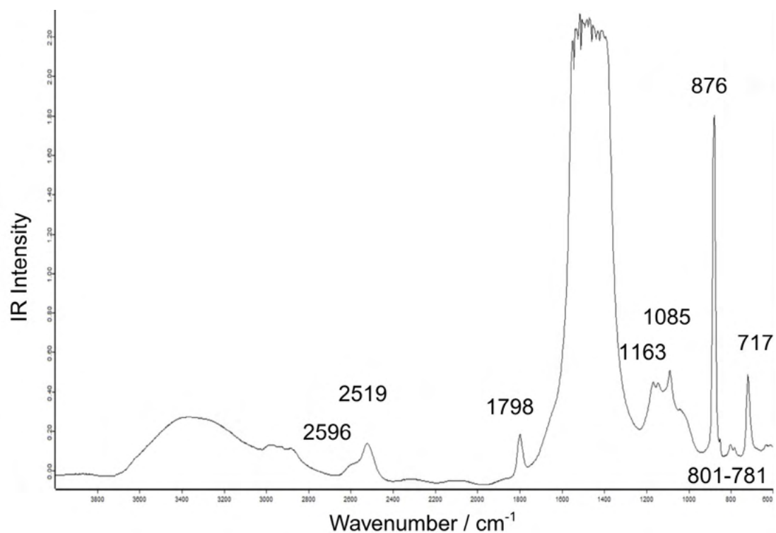
Figure 136. FT-IR spectrum of a sample collected from a bead (inv. no. I.G. 355542; Pieve d'Alpago): calcite, quartz and org. mat.
