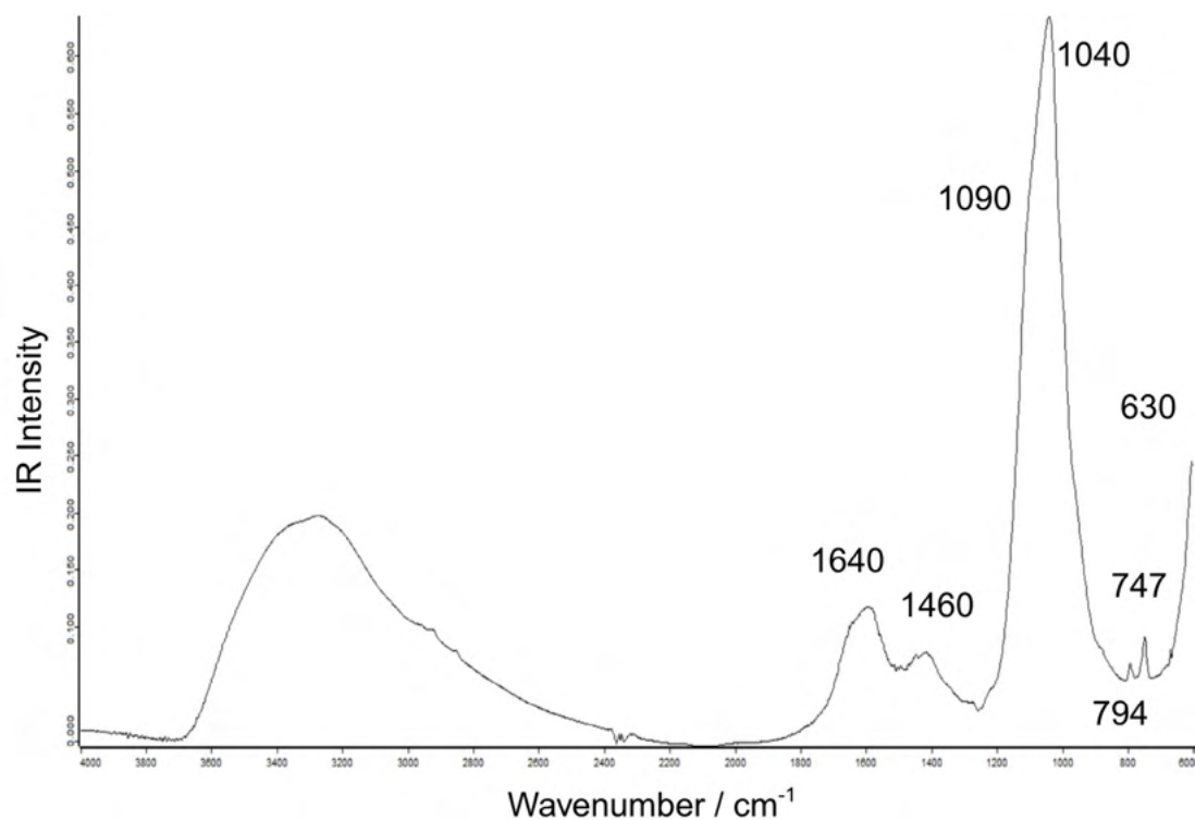
Figure 138. FT-IR spectrum of sample collected from a leech fibula with circular decoration (inv. no. St. 23751; Sesto Calende, loc. Mulini Bellaria, grave 4; Museo Civico Archeologico Sesto Calende): hydroxylapatite and organic material.
