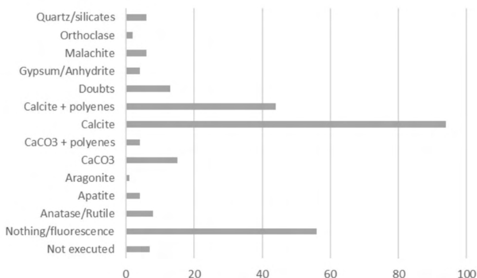
Figure 117. Inorganic compound identified by Raman analysis and abundance.
