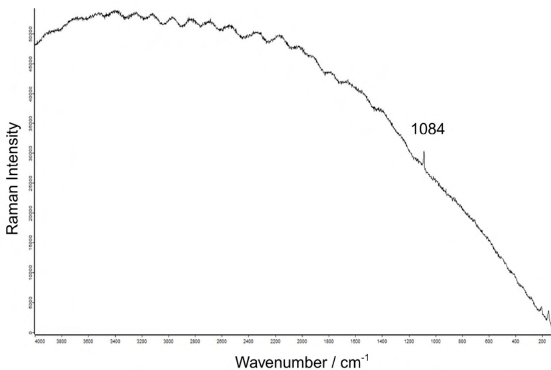
Figure 120. Raman spectrum of whitish inset on a bronze fragment from Pontecurone (AL; inv. no. 23.M.380-9.6): \text{CaCO}_3 .
