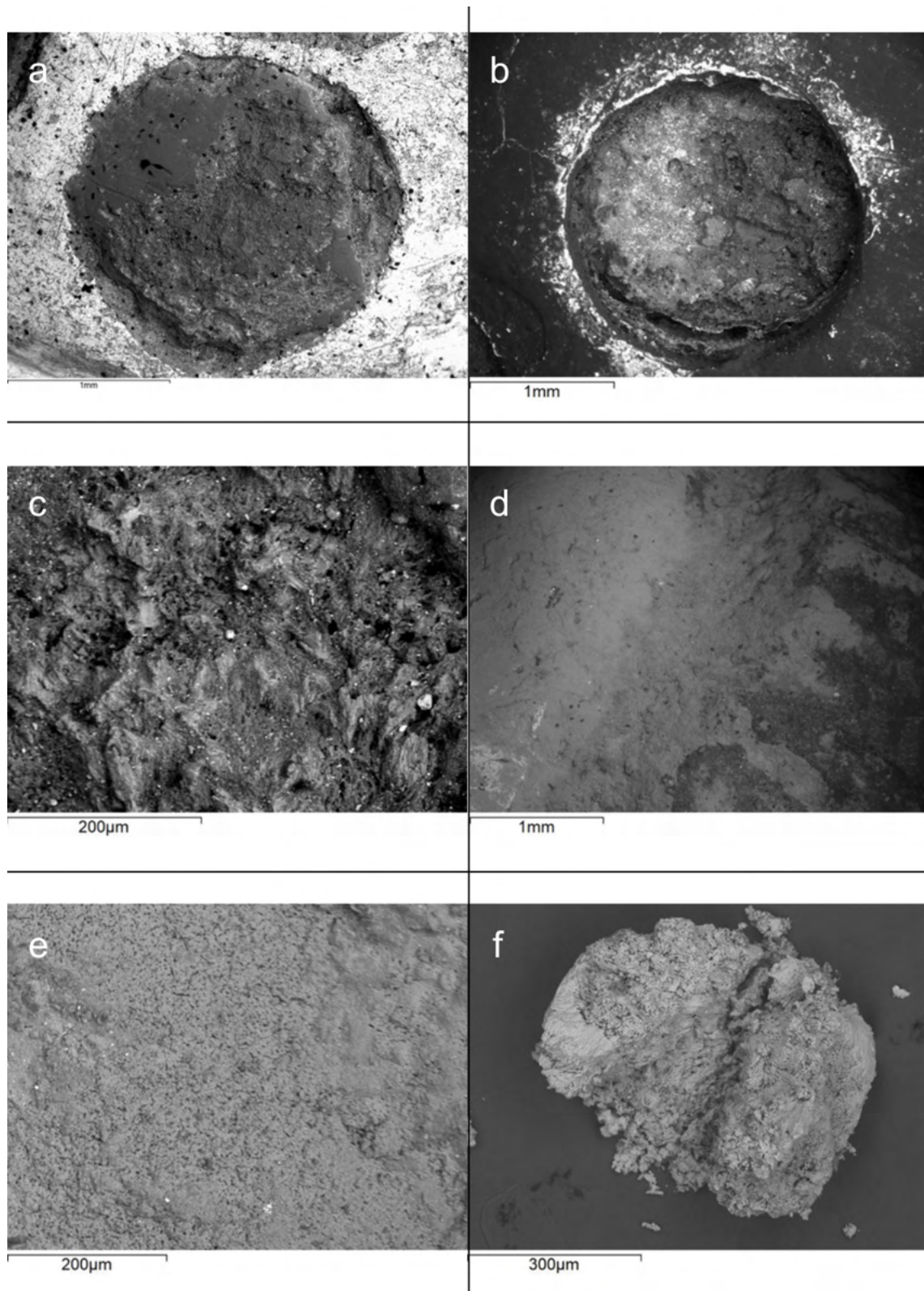
Figure 221. a) BSE-image of a circular decoration (Motto Lagone, T1); b) BSE-image of a circular decoration with high presence of Paraloid on the metal surface (Motto Lagone, T1); c) BSE-image of a circular decoration (Motto Lagone, T1): multi-branched micro-morphology; d) BSE-image of a pendant surface (Brembate Sotto, inv. no. 3016): garland-like wavy structure; e) BSE-image of an element of a composite bow fibula (Brembate Sotto, inv. no. 3052): micro-porous morphology; f) BSE-image of a sample from a circular decoration (Brignano Frascata, inv. no. C-FR-NE/2): multi-branched micro-morphology.
