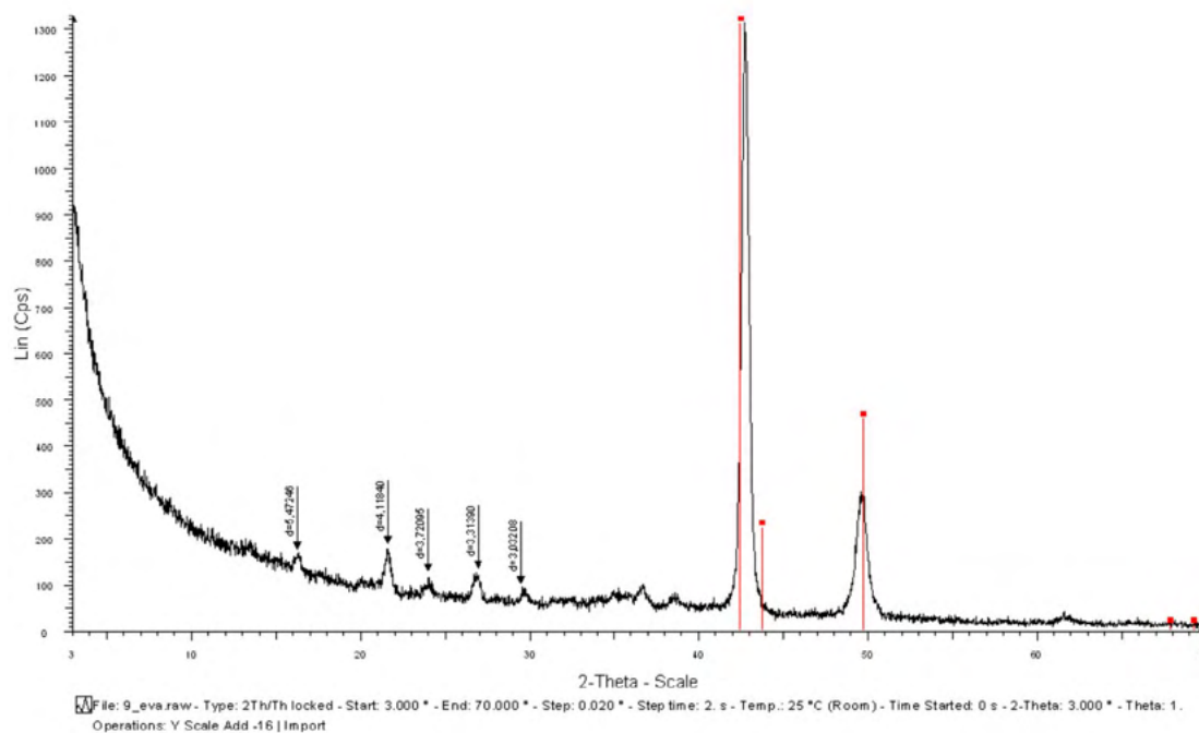
Figure 179. Diffractogram of fibula inv. no. 9 (Parre) with linear decoration: bronze ( d = 2.12 e 1.84 ) and unidentified reflections at d = 3.03 , 3.31 , 4.12 e 5.47 .
