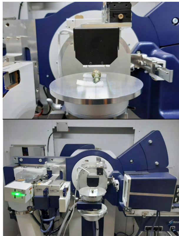
Figure 94. \mu -XRD instrumentation during the analysis of some archaeological finds.
