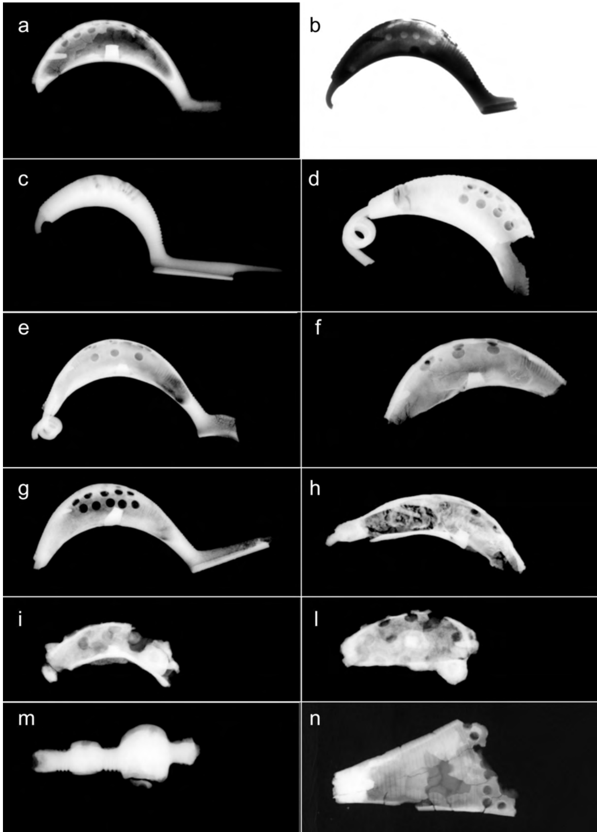
Figure 227. a) Radiography of inv. no. 868; b) Radiography of inv. no. 197; c) Radiography of inv. no. 870; d) Radiography of inv. no. 198; e) Radiography of inv. no. 944; f) Radiography of inv. no. 946; g) Radiography of inv. no. 947; h) Radiography of inv. no. 949; i) Radiography of inv. no. St. 83925; l) Radiography of inv. no. St. 83925; m) Radiography of inv. no. St. 83946; n) Radiography of inv. no. St. 83946.
