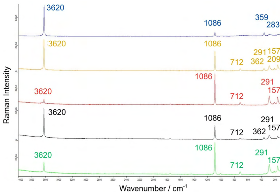
Figure 157. Comparison of the different Raman spectra of burnt corals 9 months after combustion, from top to bottom: zero (blue), one (orange), two (red), three (black), four (green).
