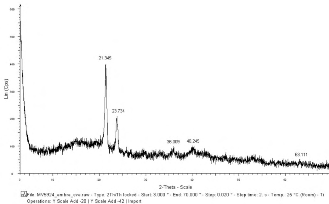
Figure 149. Diffractogram of the object inv. no. MV5924 (presumably amber by microscopic observation; unknown provenance, Musei Civici Villa Mirabello Varese): reflections attributable to wax (GAILLARD et al. 2011; SCHOENING 1980), instead of amber (PAKUTINSKIENE et al. 2007).
