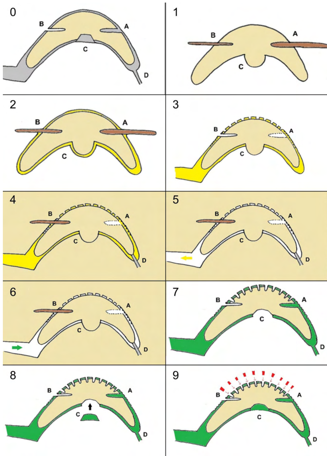
Figure 213. 0) Schematisation of observations made on archaeological artefacts; 1) Clay core; 2) Beeswax coverage; 3) Modelling the wax model; 4) Preparation of the mould; 5) Wax removal; 6) Bronze casting; 7) Mould opening; 8) Cap insertion; 9) Coral elements insertion.
