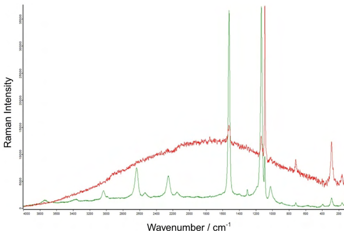
Figure 91. Raman spectra of the same modern coral sample (ball_800; C. rubrum ) with green laser (532 nm) in green and with red laser (633 nm) in red: in the first case, the peaks relating to the presence of polyenes clearly predominate over those of calcite, while in the second case the calcite signals are preponderant.
