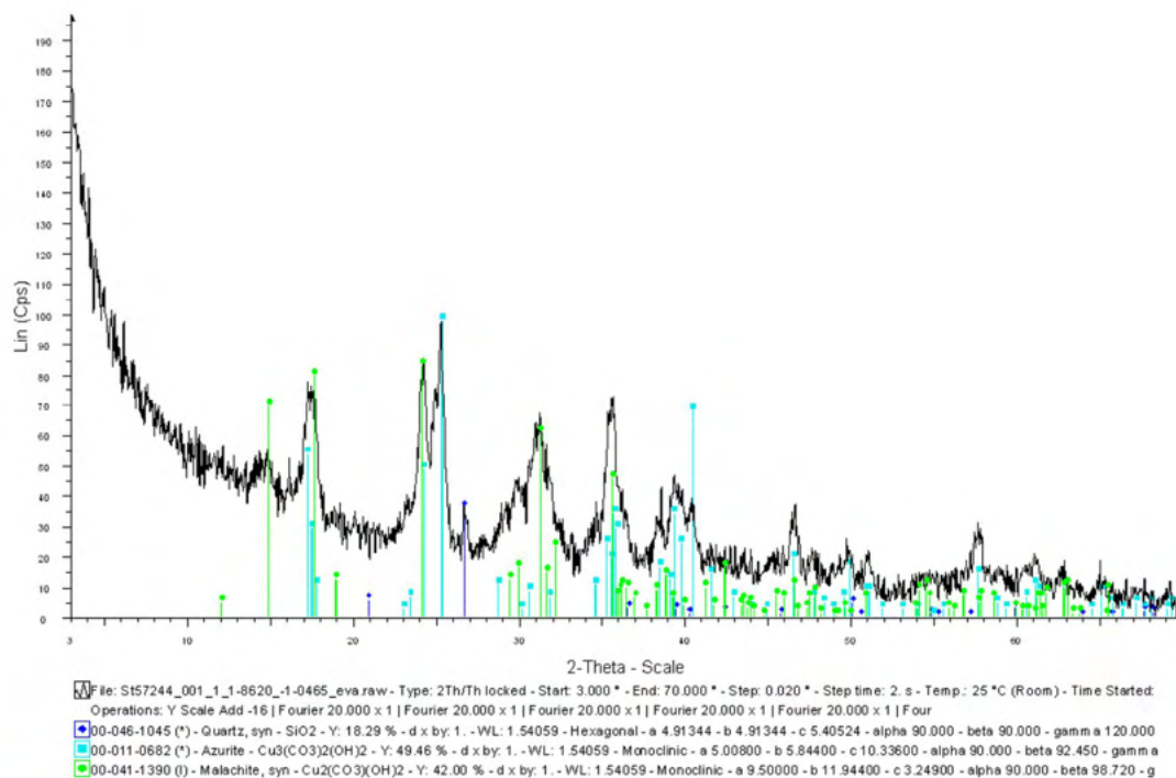
Figure 181. Diffractogram of fibula inv. no. St. 57244 (Como, via Isonzo): azurite (light blue), malachite (green) and quartz (blue).
