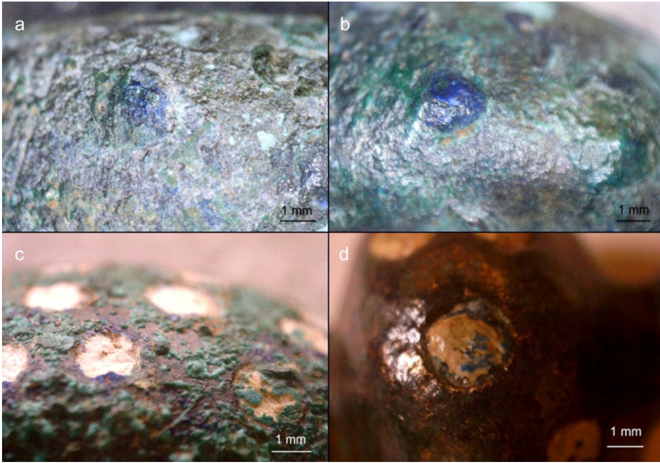
Figure 220. a) Montebelluna, loc. Posmon; Leeche fibula with circular insets (inv. no. I.G. 304780, Montebelluna Museum): blue metallic alteration products on the circular decoration; b) Montebelluna, loc. Posmon; Leeche fibula with circular insets (inv. no. I.G. 304784, Montebelluna Museum): blue metallic alteration products on the circular decoration; c) Pieve d'Alpago; Leeche fibula with circular insets (inv. no. I.G. 312348, SABAP): blue metallic alteration products on the circular decoration; d) Cavarzano, Masiera; Leeche fibula with circular insets (inv. no. 217, Museo Civico Belluno): blue metallic alteration products on the circular decoration.
