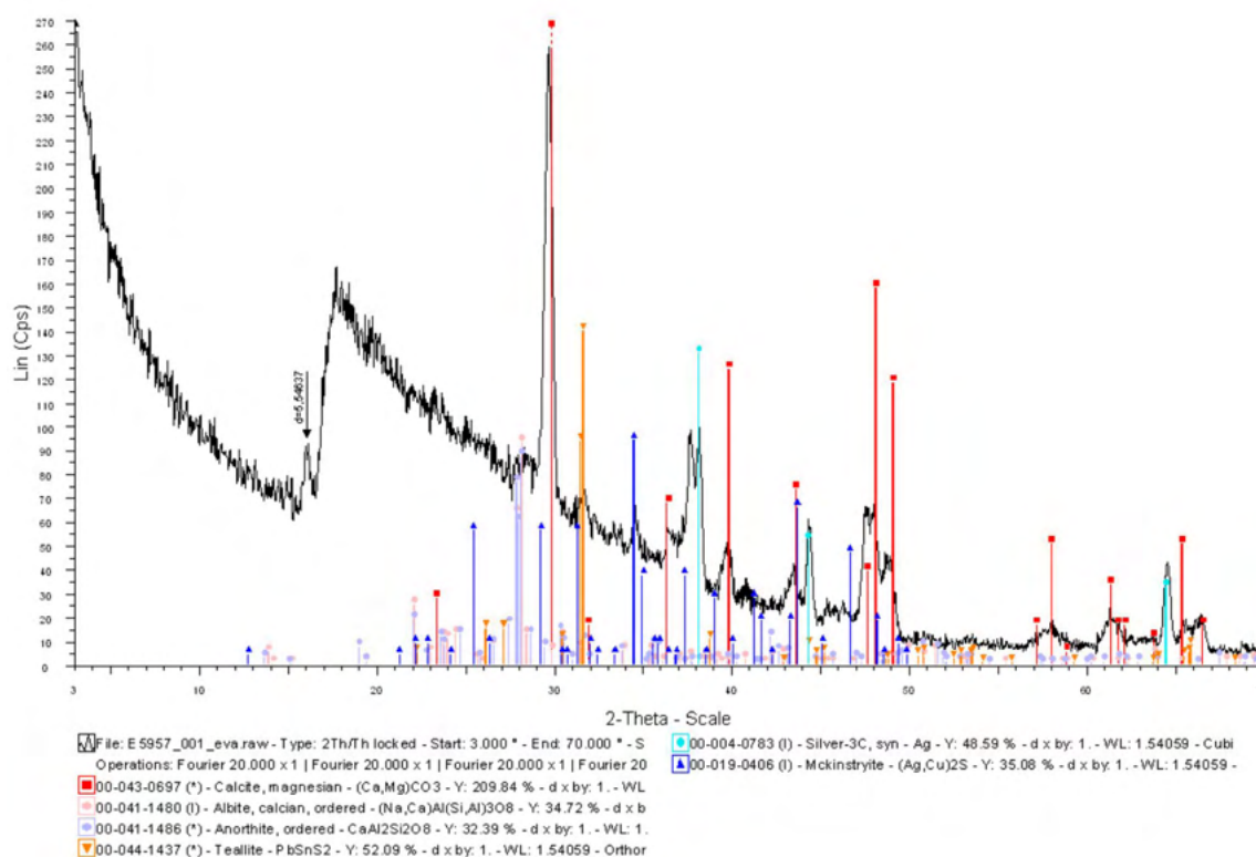
Figure 178. Diffractogram of composite fibula inv. no. E5957 (Como): Mckinstryite (blue), silver (light blue), Mg-calcite (red), teallite (orange), albite (pink), anorthite (purple).
