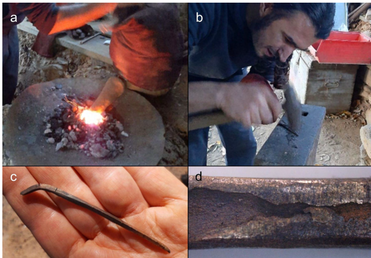
Figure 212. a) Reheating the semi-finished product by reverse tempering; b) Processing by hammering; c) Breaking defect during hammering; d) Detail of the folding of the edges of the semi-finished product.
