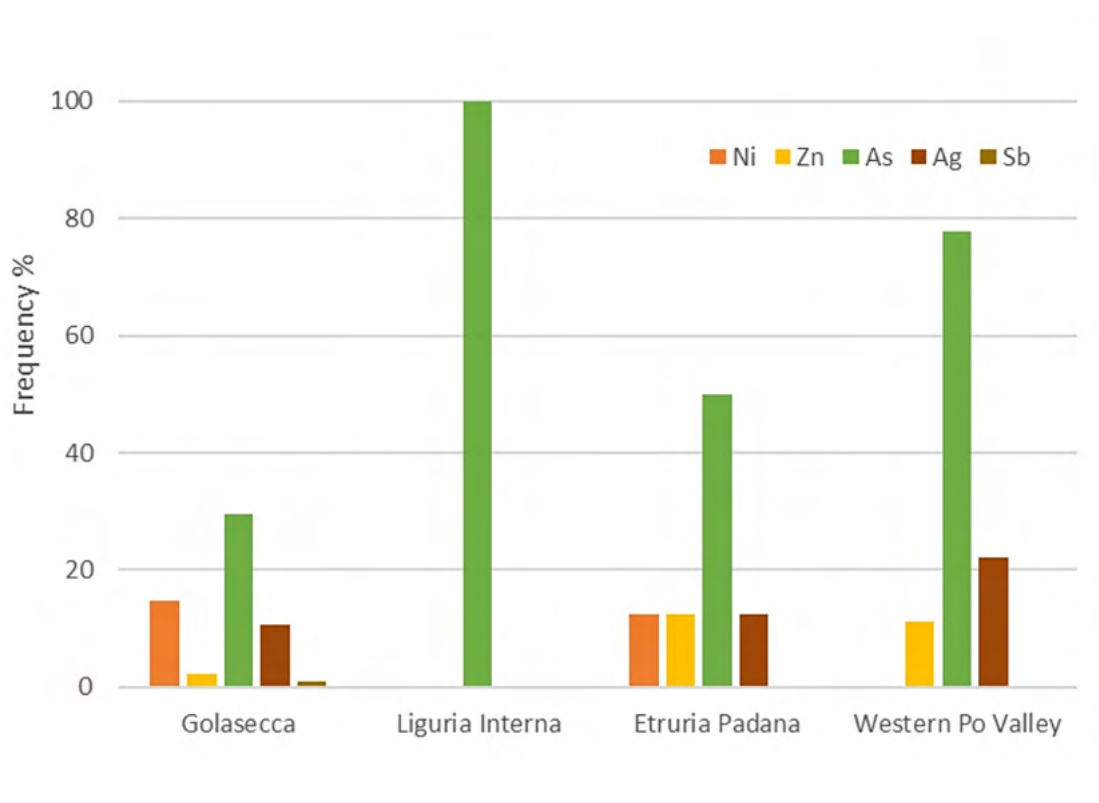
Figure 192. Frequency % of the most significant trace elements in relation to main geographical-cultural areas.
