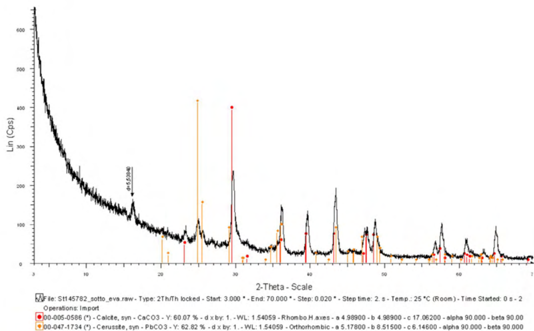
Figure 185. Diffractogram of bucket pendant inv. no. St. 145782 (Forcello di Bagnolo San Vito): cerussite (orange) and calcite (red).
