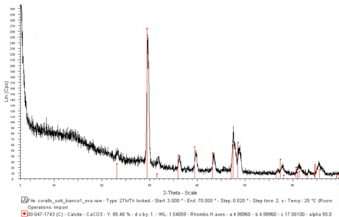
Figure 105. \mu -XRD diffractograms of 'r_c_L' (Ligurian white coral): calcite.
