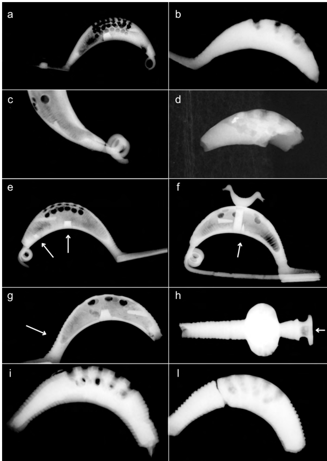
Figure 202. a) Detail of the bow with terracotta core and internal metal elements (tomb 1, Motto Lagone, Arona); b) Detail of the full-arch of the fibula inv. no. St. 114083 (Como); c) Detail of the pin insertion point in the bow body (inv. no. 944, Castelletto Ticino – Vigevano?); d) Detail of the hole left by the inner element on the upper-foot-side (D2065, Golasecca); e) Leech fibula with terracotta core with double ventral side support pin (inv. no. CT728, Castelletto Ticino); f) Leech fibula with terracotta core with orthomorph internal element (inv. no. D2773, Castelletto Ticino); g) Alternated linear decoration (inv. no. St. 879, Como); h) Fibula foot with globe and vase-shaped final part (inv. no. St. 83937, Pombia); i) Full-arch fibula, detail of superficial corrosion (inv. no. St. 2208, Como); l) Full-arch fibula with recomposed fracture (inv. no. St. 2206, Como).
