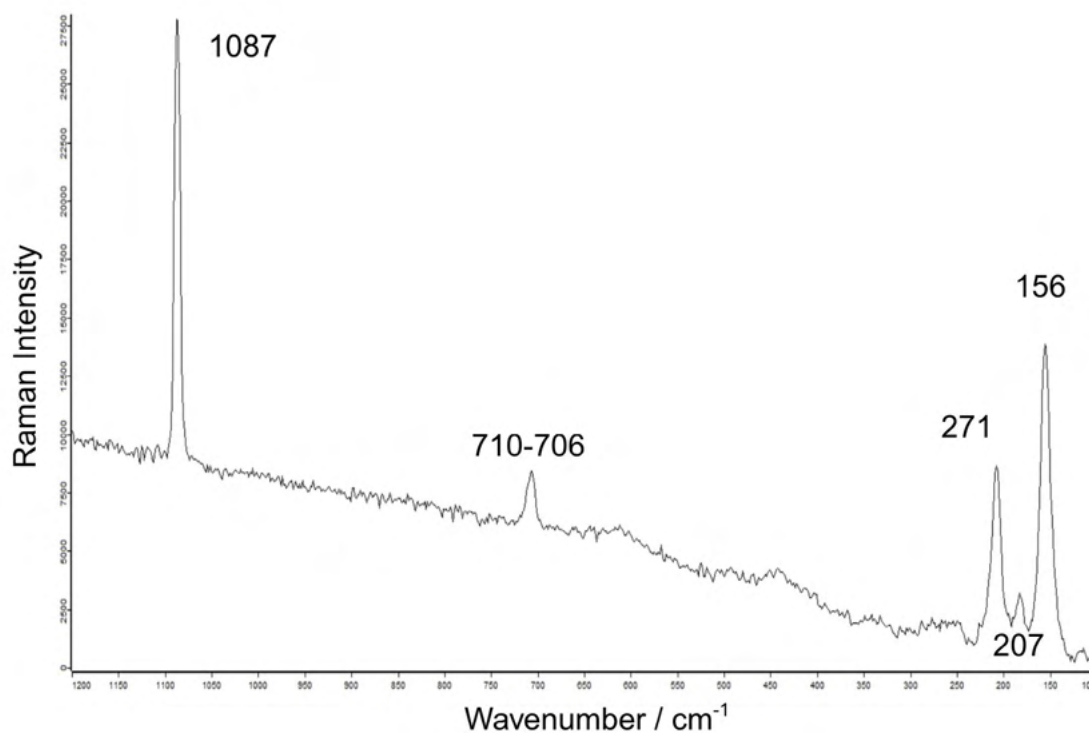
Figure 121. Raman spectrum of whitish linear decoration on a grooming tool (tweezer) from Piovego (PD; T95.10): detail of the part of interest, showing characteristic peaks of aragonite.
