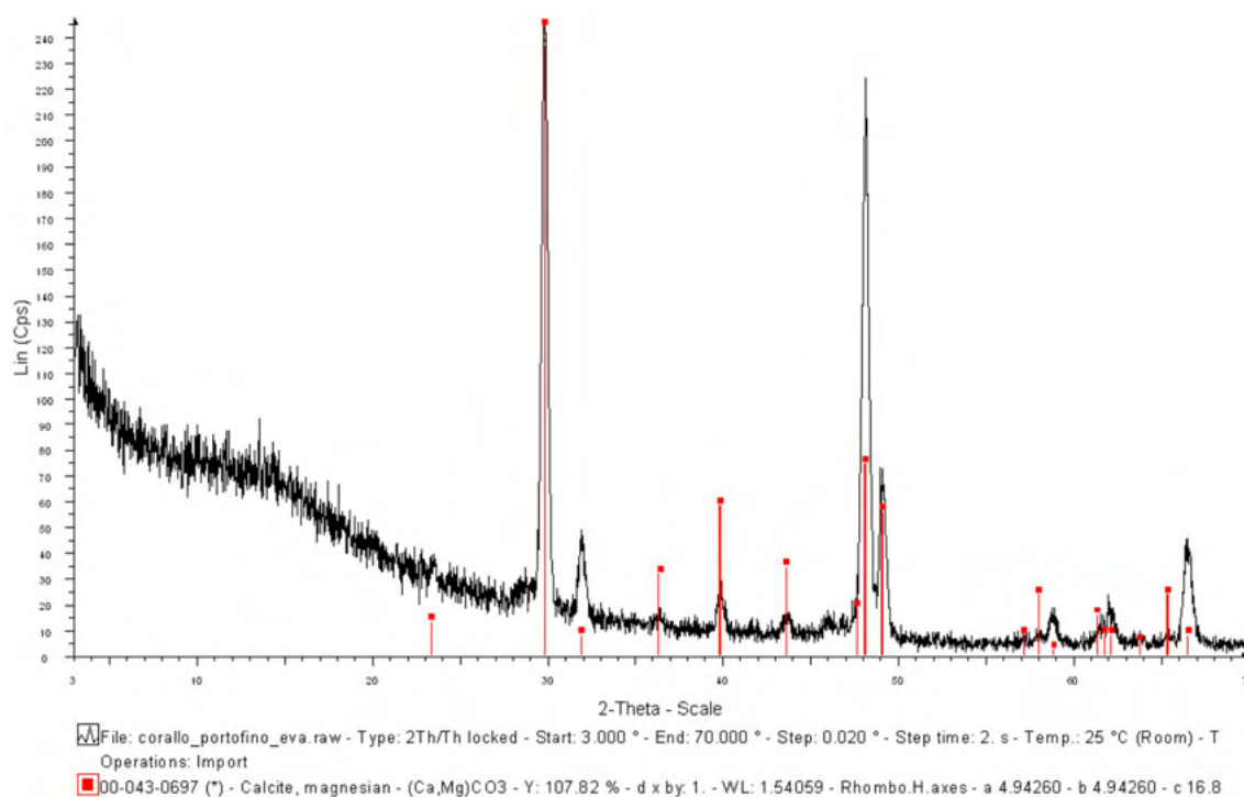
Figure 104. \mu -XRD diffractogram of 'r_Cr_L' (ligurian C. rubrum ): Mg-calcite.
