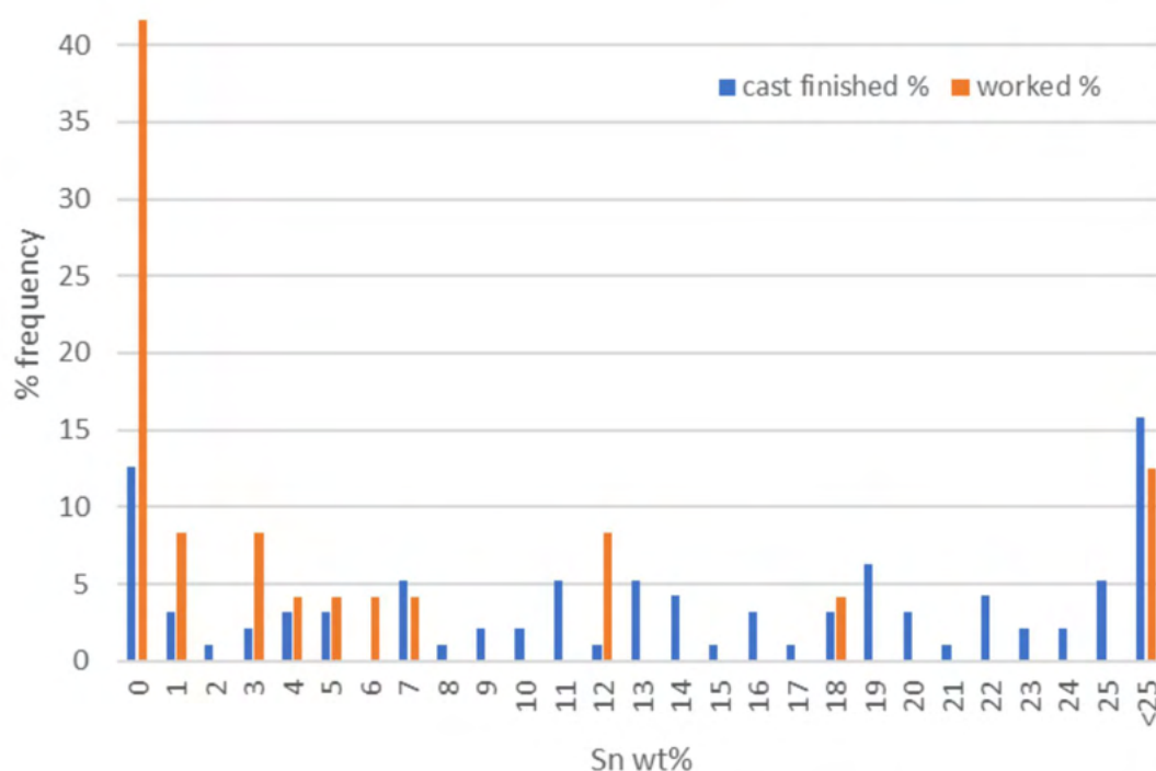
Figure 188. Sn wt% content frequency for cast-finished and worked after casting objects: each column counts the number of objects having Sn in a concentration range of 1% by weight.
