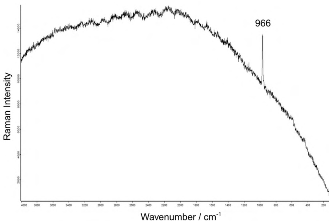
Figure 127. Raman spectrum of whitish Longone al Segrino type pendant from Como, Ca' Morta, grave 200 (inv. no. St. 124142; magnification 10X, filter d 0.3): apatite. Further points of analysis on the same find show the clear presence of calcite; the signs of apatite are probably attributable to contamination by bone tissue referable to the deceased.
