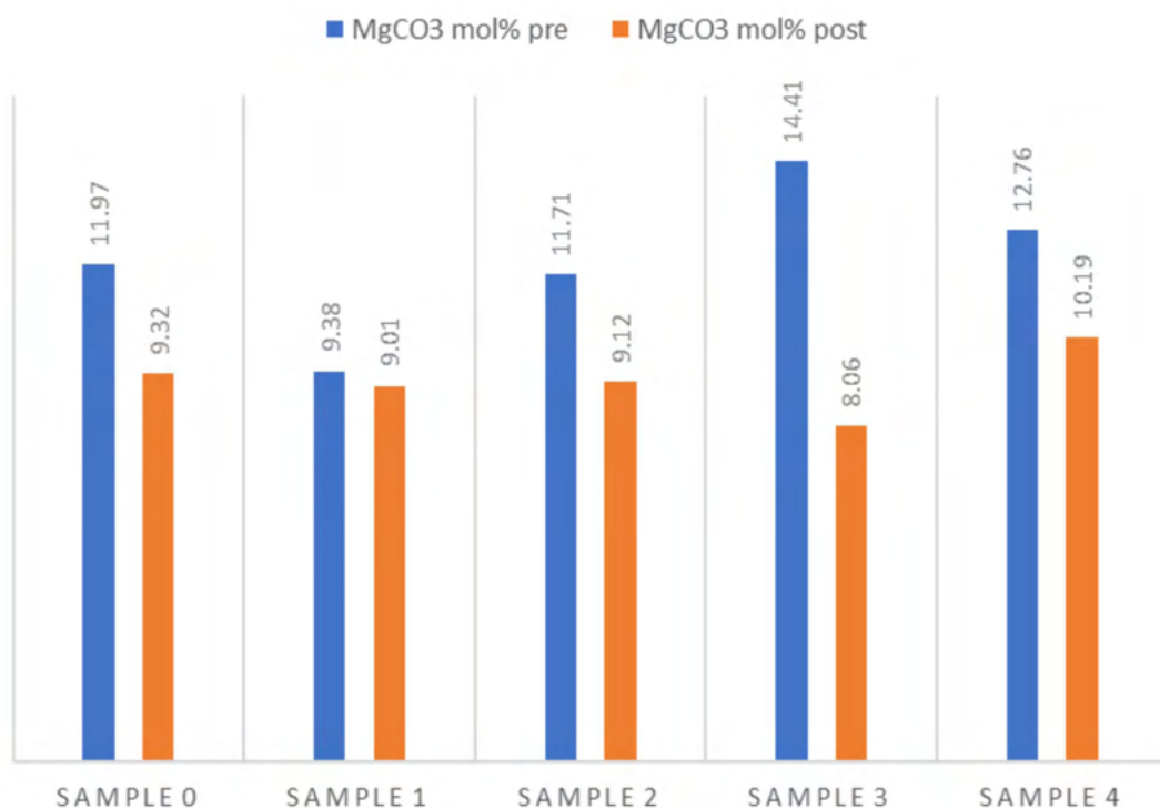
Figure 159. Graph of the variation in magnesium content in calcite before and after burning coral samples.
