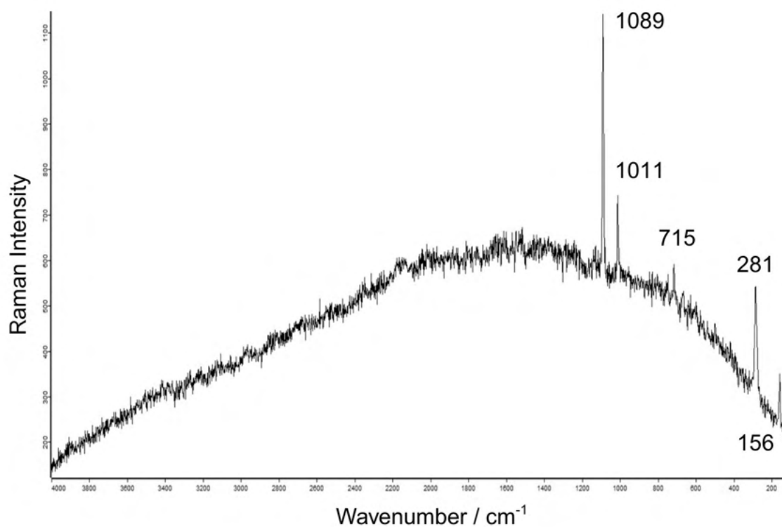
Figure 125. Raman spectrum of whitish circular decoration on Golasecca leech fibula (inv. no. D2065; magnification 10X, filter d 0.3): calcite and anhydrite.
