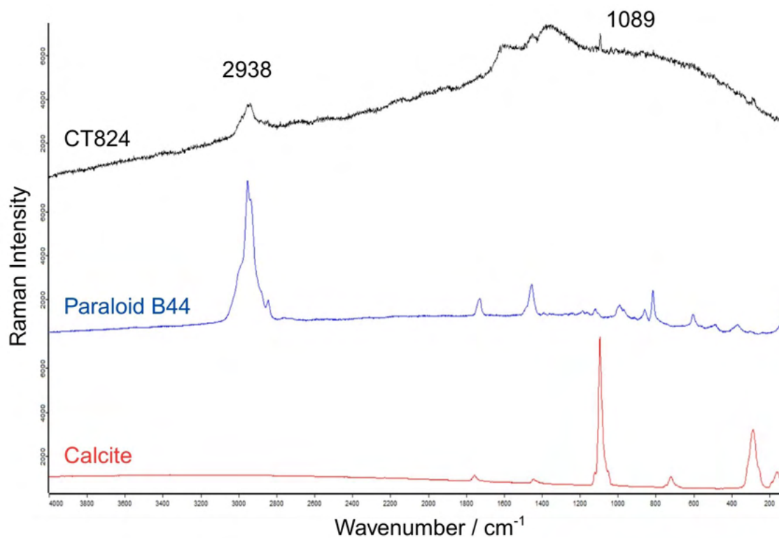
Figure 129. Comparison of Raman spectra obtained from analysis of the find CT824 in black, Paraloid B44 in blue and calcite in red; 10X magnification, D0.3 filter.
