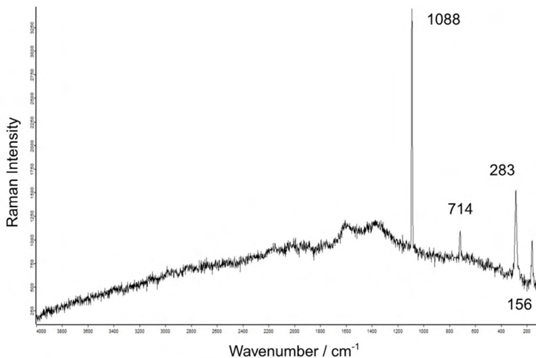
Figure 119. Raman spectrum of whitish circular decoration on Como (Ca' Morta, Rebbio, Cava Ballerini) leech fibula (inv. no. St. 879; magnification 10X, filter d 0.3): calcite.
