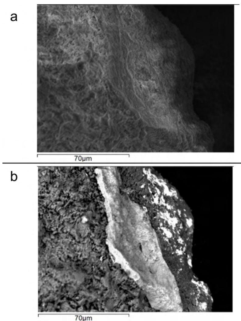
Figure 96. Archaeological decoration sample - copper and lead 'crust' on Ca/Mg-based material, high vacuum: a) image obtained with secondary electron detector (ESE); b) image obtained with backscattered electron detector (BSE).
