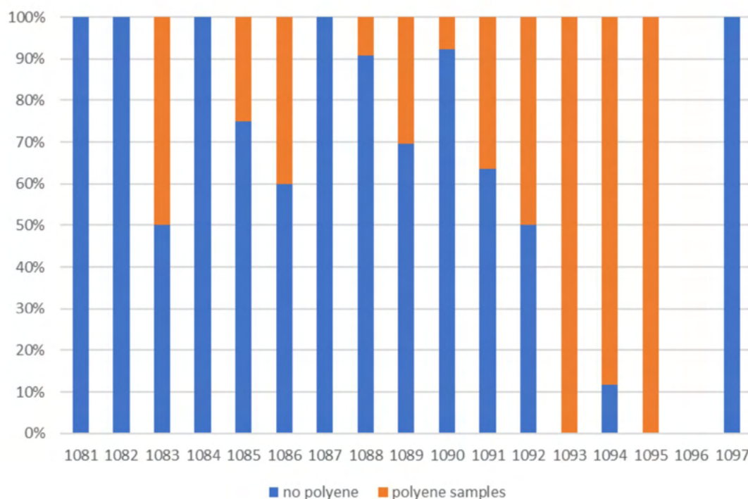
Figure 122. Graph showing the frequency of different values for the main carbonate peak ( \nu_1 ) in spectra with (in red) and without (in blue) polyenes, as a percentage of the total (see Appendix 2, Tab. 38).
