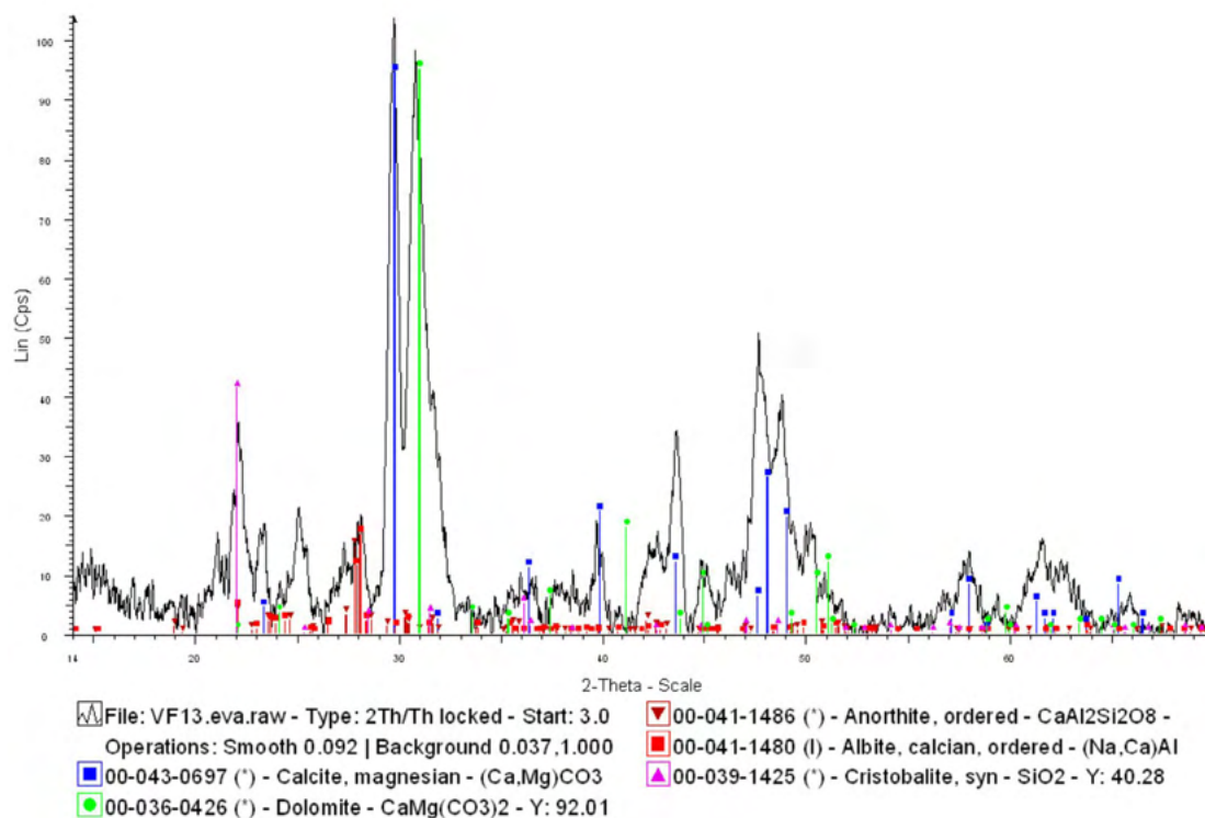
Figure 143. Diffractogram portion of the sample VF13 (collected by finds St. 51877, Villa del Foro): main reflections of HMC (blue) and dolomite (green) visible, together with other crystalline phases.
