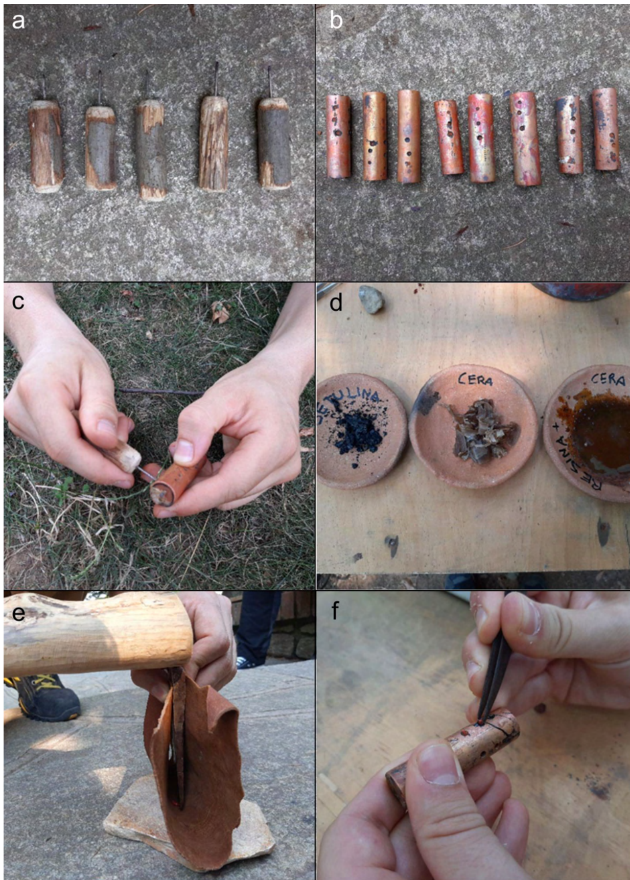
Figure 203. a) Drilling tools; b) Copper and clay tests; c) Deepening the holes in the inner core; d) Binders: birch pitch, beeswax and a mixture of beeswax and pine resin; e) Cutting tests with bronze tool; f) Insertion of the coral inset.
