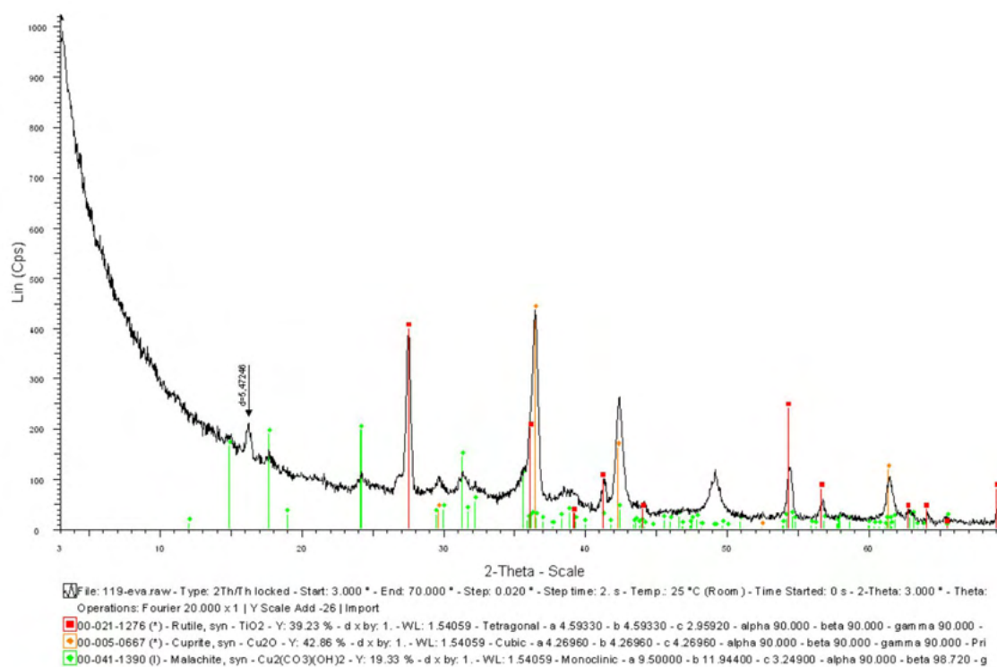
Figure 148. Diffractogram of the fibula inv. no. 199 (Parre): in red rutile reflections, in orange cuprite reflections, in green doubtful malachite reflection.
