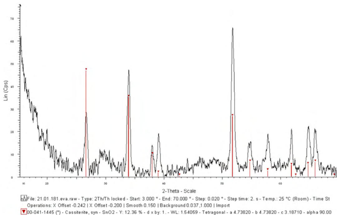
Figure 187. Portion of the diffractogram obtained on the fibula's foot inv. no. 2021.01.181 (Gropello Cairoli, loc. Santo Spirito): cassiterite.
