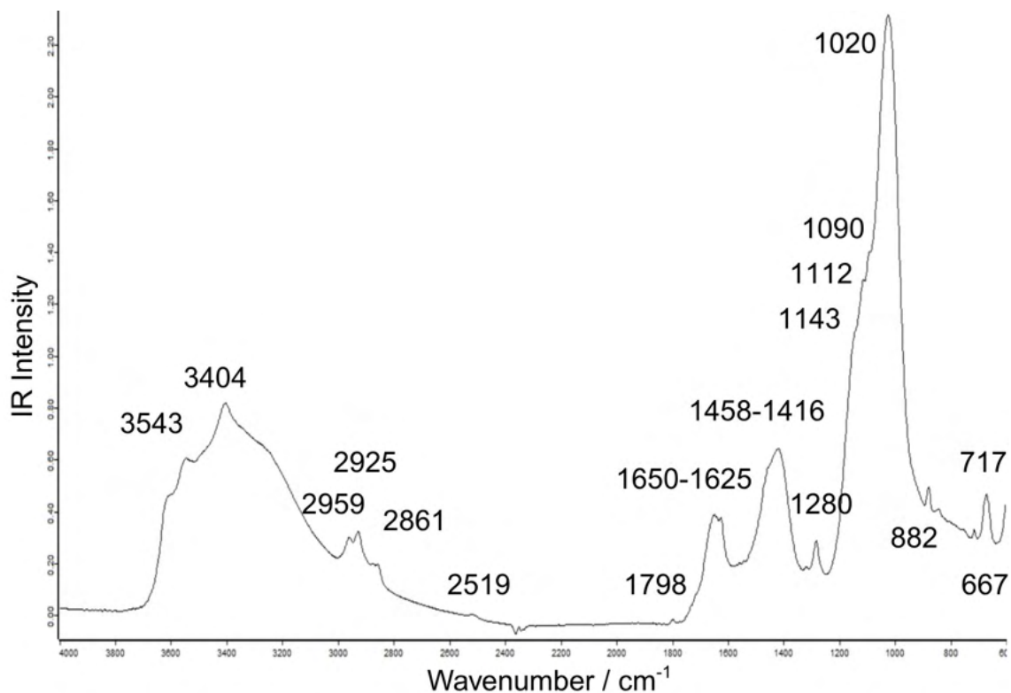
Figure 137. FT-IR spectrum of sample collected from a leech fibula with circular decoration (Collezione Bellini; Museo Civico Archeologico Sesto Calende): calcite, gypsum, silicate, org. mat.
