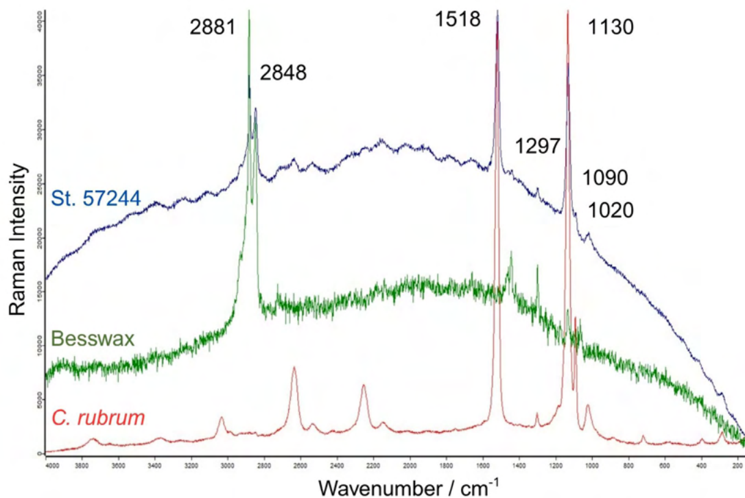
Figure 130. Comparison of Raman spectra obtained from analysis of the circular decoration of find St57244 in blue, beeswax in green and Corallium rubrum in red; 10X magnification, D0.3 filter.
