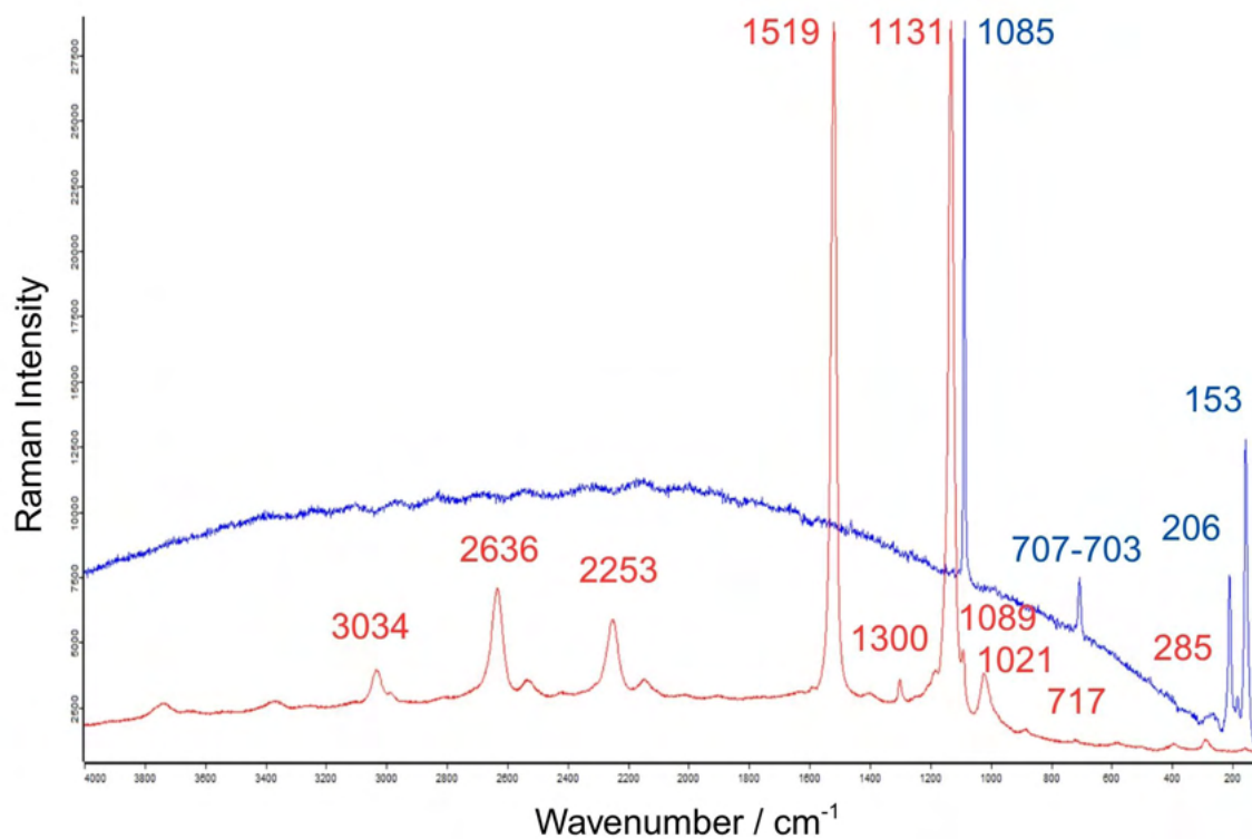
Figure 100. Comparison between Raman spectra collected on sample 'r_Cr_Si' in the red (red) and white (blue) portions, respectively composed of calcite with polyenes and aragonite; 532 nm green laser, extended range, 6 seconds for 6 cycles, 10x magnification, D0.6 filter.
