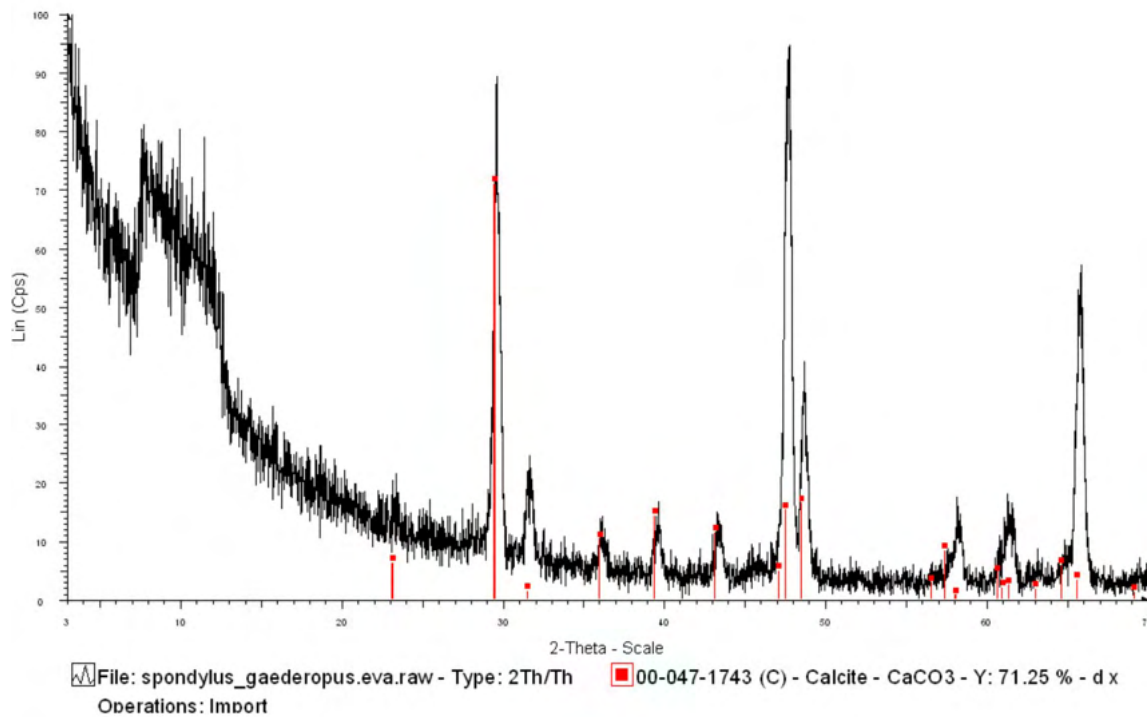
Figure 106. \mu -XRD diffractograms of 'r_Sg_Sa' ( Spondylus gaederopus ): calcite.
