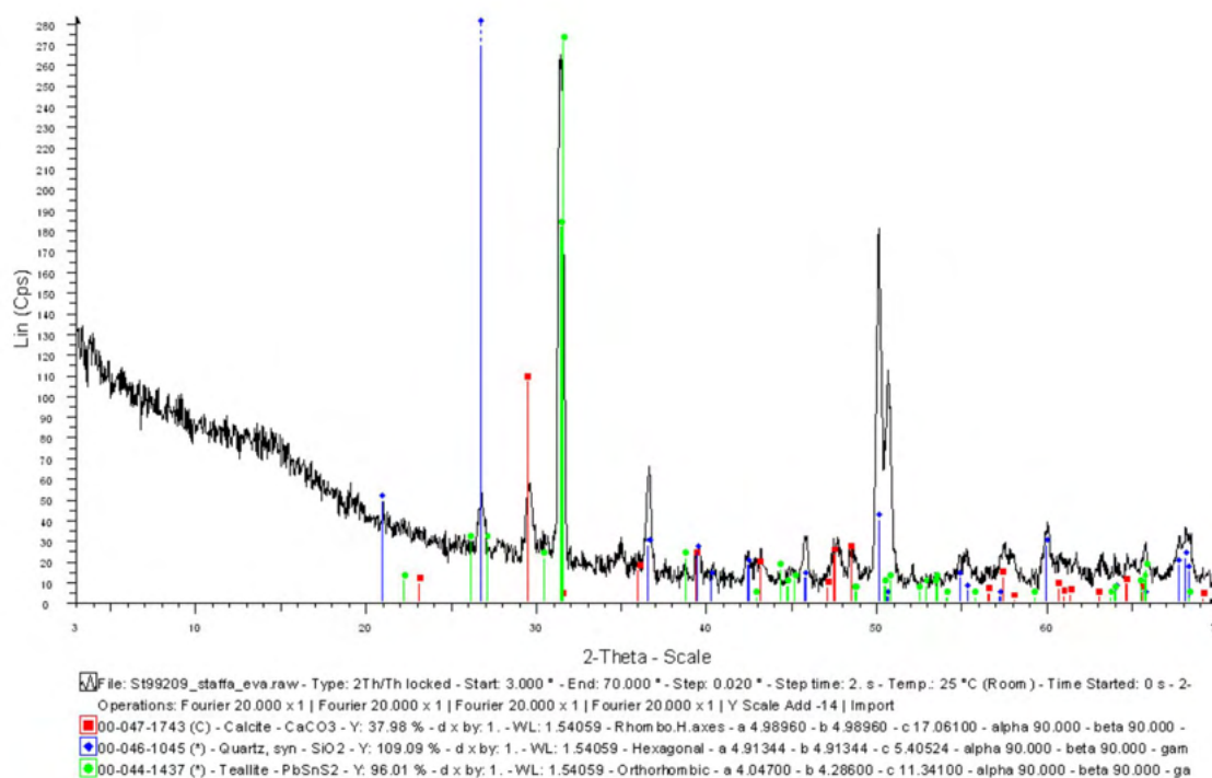
Figure 186. Diffractogram of a point on the foot of the fibula inv. no. St. 99209 (Forcello di Bagnolo San Vito): teal-lite (green), calcite (red) and quartz (blue).
