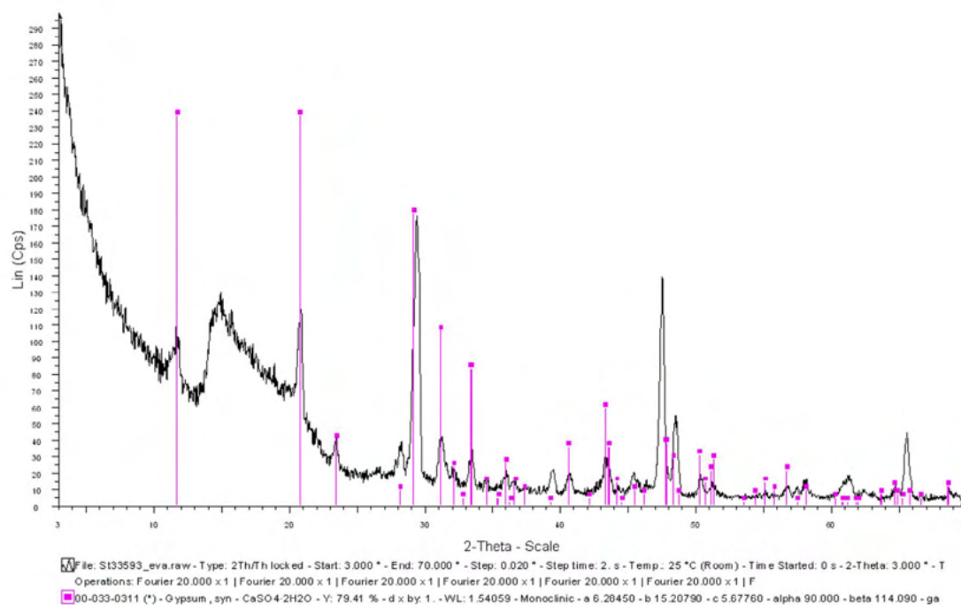
Figure 145. Gypsum diffractogram of the pendant inv. no. St. 33593 (Como, grave 302).
