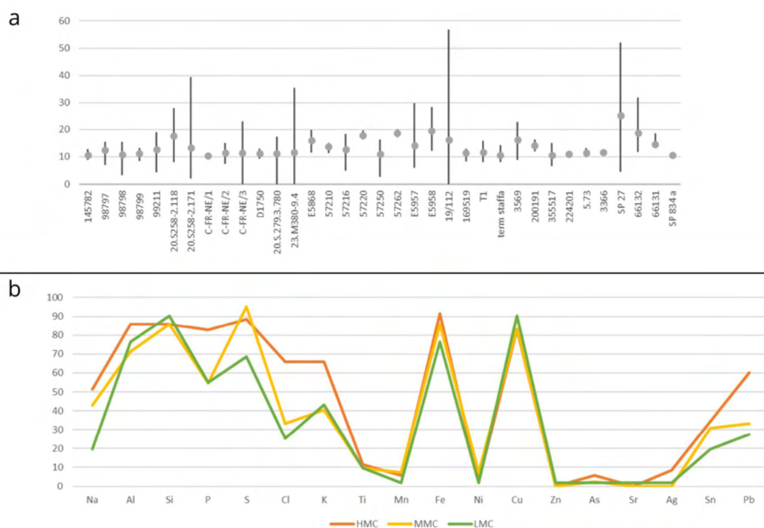
Figure 153. a) HMC samples: Mg-content variation in each sample (bar indicates the variation between minimum and maximum value) and average value (point indicates the average value of all the points of analysis on the sample); b) Graph of the occurrence (as a percentage of the total) of minor elements in calcites with different Mg-content.
