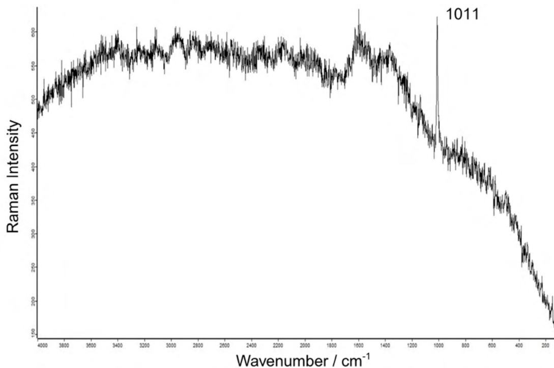
Figure 126. Raman spectrum of whitish Longone al Segrino type pendant from Como, Ca' Morta, grave 302 (inv. no. St. 33593; magnification 10X, filter d 0.3): gypsum.
