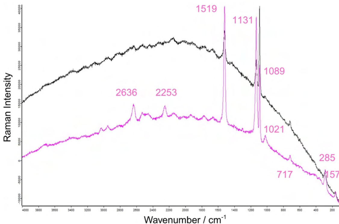
Figure 101. Comparison between Raman spectra of the Sardinian coral pendant (w_pCr_Sa) in the white portion (in black) and the pink portion (in fuchsia); 532 nm green laser, extended range, 6 seconds for 6 cycles, 10x magnification, D0.6 filter.
