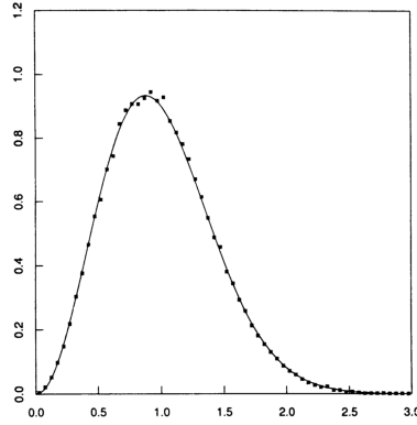
Figure 25.4 The normalized distribution of the spacings of 10^5 zeros of the Riemann function \zeta(z) on the line \text{Im} z = \frac{1}{2} and the Wigner surmise (from: A. M. Odlyzko, On the distribution of spacings between zeros of the Zeta function, Mathematics of Computation 48 (1987) 273–308).
