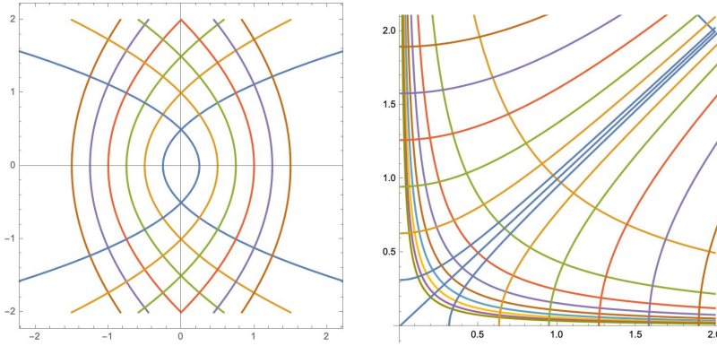
Figure 5.3 The quadratic map w = z^2 . Left: the confocal parabolas in w -plane are the images of the coordinate square grid x - y in z -plane. Right: the hyperbolas in z -plane are the pre-images of the coordinate square grid u - v in w -plane (only a quadrant is shown).
