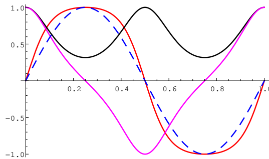
Figure 15.1 The functions \operatorname{sn}(4Kx|k) (red), \operatorname{cn}(4Kx|k) (fuchsia), \operatorname{dn}(4Kx|k) (black) with k = 0.9 and, for comparison, the function \sin(2\pi x) (dashed). As k increases, the maxima and minima of \operatorname{sn} become more rounded.
