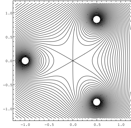
Figure 6.1 The equipotential lines of 3 unit charges (i.e. three wires with same linear charge crossing the plane).
