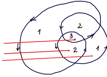
Figure 7.1 Indices of an oriented curve. To evaluate the index in a patch, fix a point in it, draw a half-line left from the point, and count the crossings from above ( N_+ ) and from below ( N_- ). The index in the patch is N_+ - N_- .
